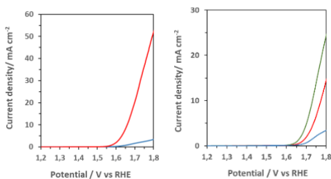
Figure 1. (left) linear sweep voltammetry comparison of rGO-Ni in KOH with Fe impurities (red) and purified (blue); (right) OER activity comparison of rGO-Ni (blue), rGO-(98Ni/2Fe) (red) and rGO-(90Ni/10Fe) (green) in KOH purified.
