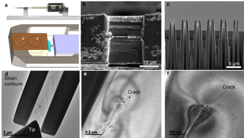
Overview of the TEM in-situ setup. (a) TEM holder (b) SEM top view of the sample after being thinned. (c) SEM front overview of the DCBs (d) TEM view of the indenter and the DCB and (e) and (f) frames obtained during the DCB splitting showing at different magnifications the crack propagating stably.
