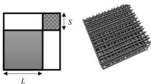
Figure 1 The three allowed tiles (left). A 3D model of the Fibonacci square quasicrystal (right).
