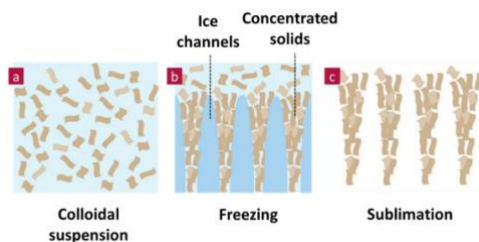
Figure 1. Freeze-casting process of graphene oxide colloidal suspension and nickel-iron particles to obtain a porous structure of concentrated solids.
