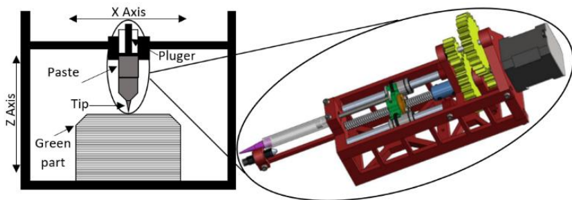
Figure 1. Schematic diagram of the DIW process (left) and CAD model of the printer head with syringe and nozzle (right).
